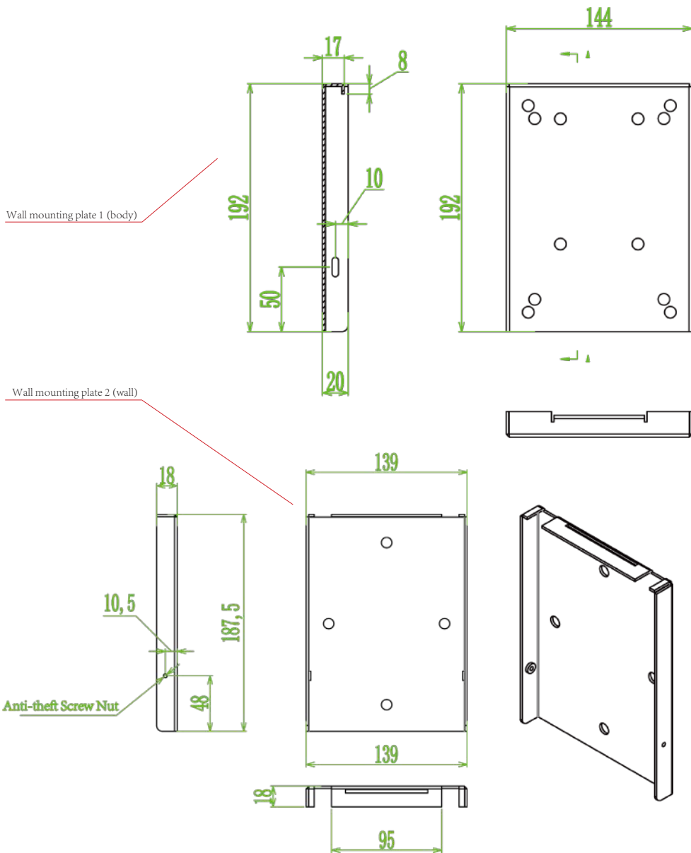
Wall mounting plate drawing (mounting plate included in package)
